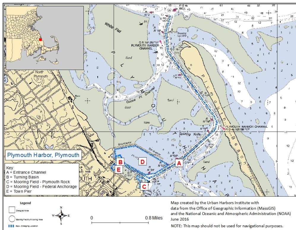
Figure 17: Dredging in Plymouth Harbor
